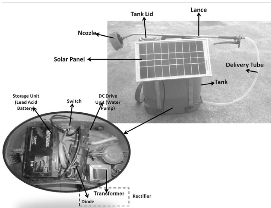
Fig 1: Developed Solar Operated Sprayer
