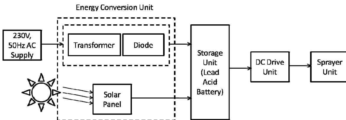
Fig 2: Block Diagram of the developed Solar Sprayer
