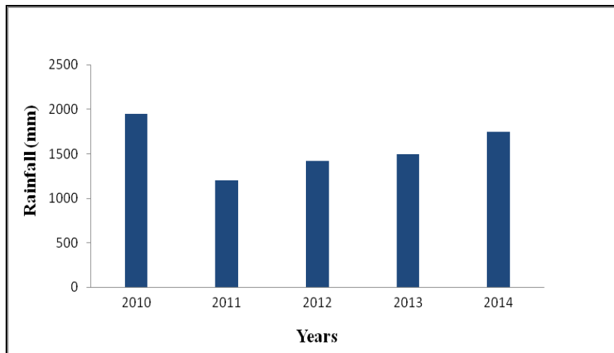
Fig 3: Mean annual rainfall of Gera District area from 2010-2014 (National Meteorology Agency, Jimma Branch, 2015).
