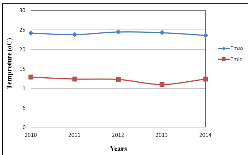
Fig 2: The mean annual Min and Max temperature of Gera Woreda (Afalo area) from 2010-2014 (National Meteorological Agency, Jimma Branch, 2015).
